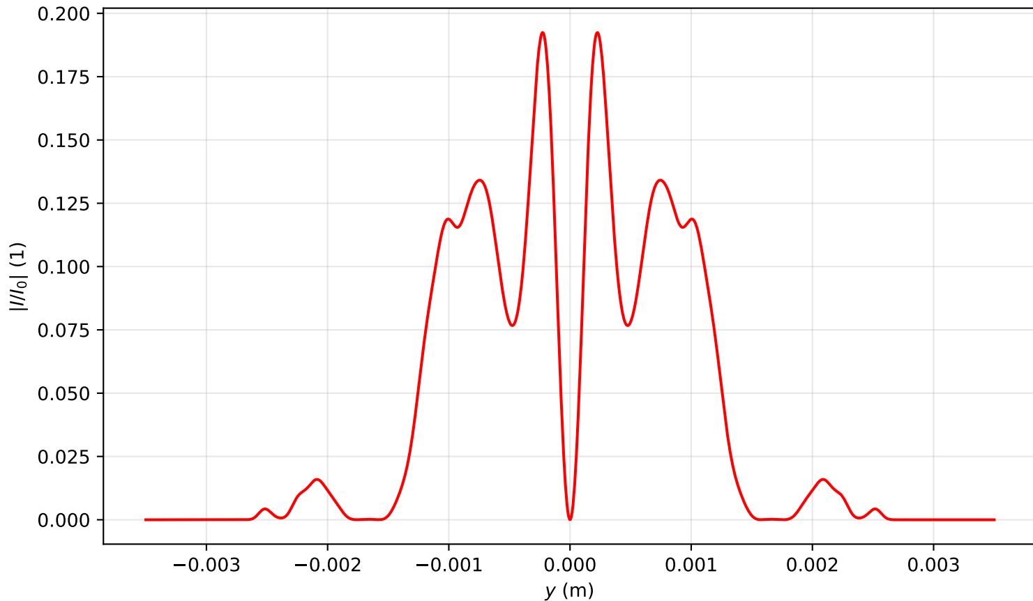
Intensity profile I(x=0, y, z=1.751)/I_0 , \text{Pin}=9.0\text{Pcr} , artificial time
